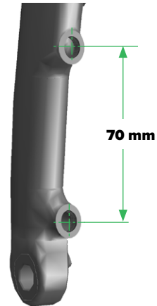
Thru Bolt Fork
