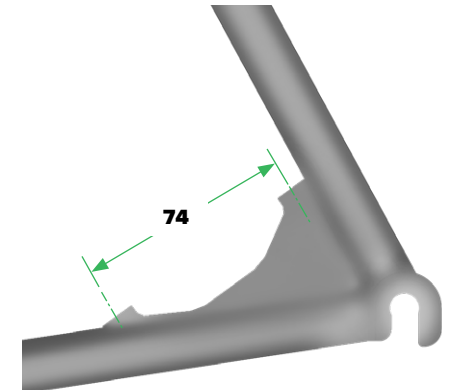
Chainstay Mount
