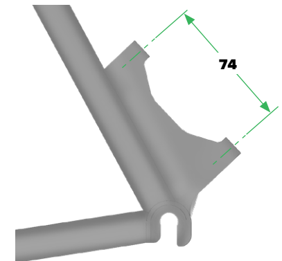
Seatstay Mount
