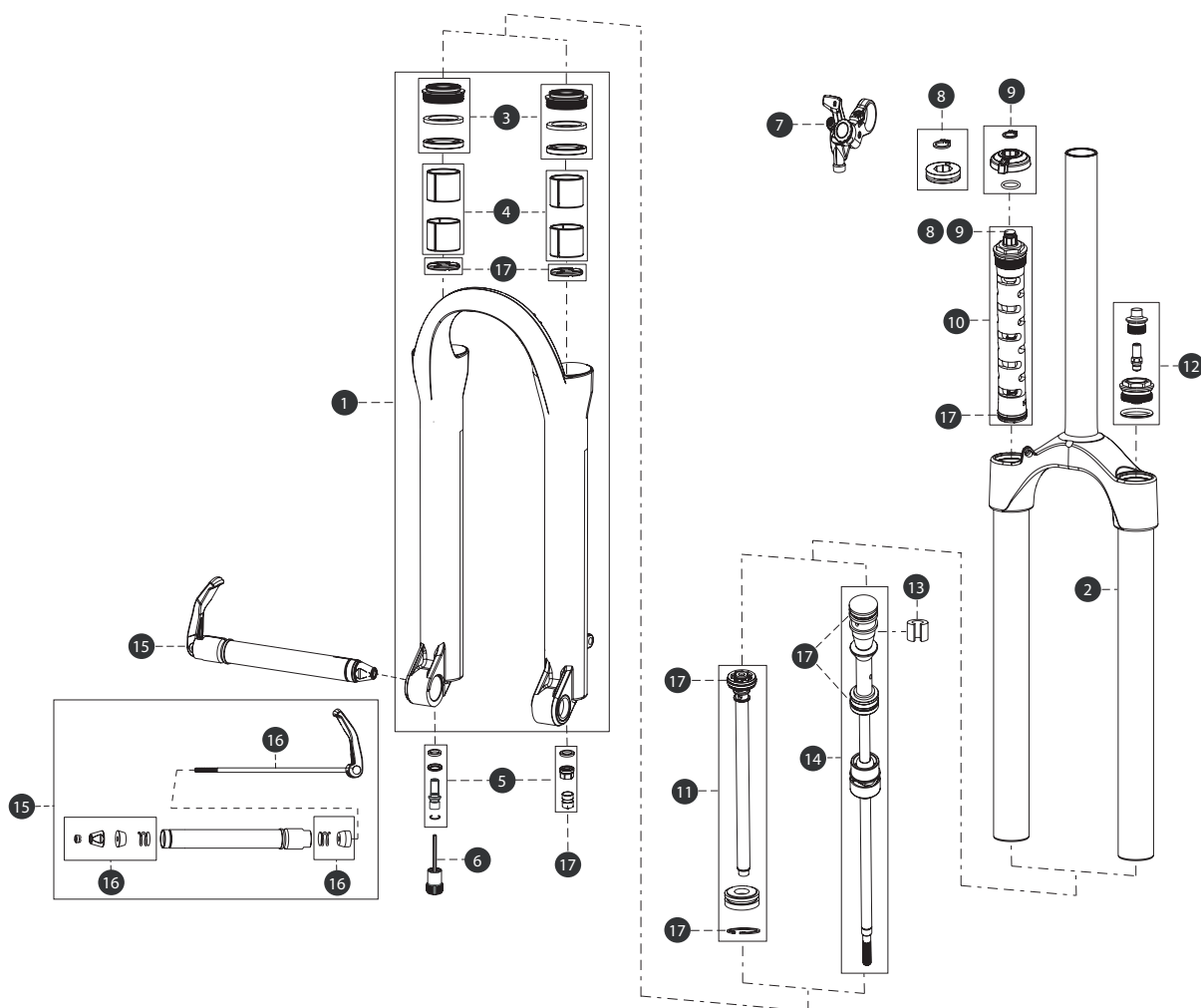
All-Travel Spacer Configurations (#13) Two All-Travel Spacers (10mm) = 120mm One All-Travel Spacer (10mm) = 130mm No All-Travel Spacer = 140mm
