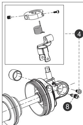
ARIO 2.R/REMOTE TOP-PULL
